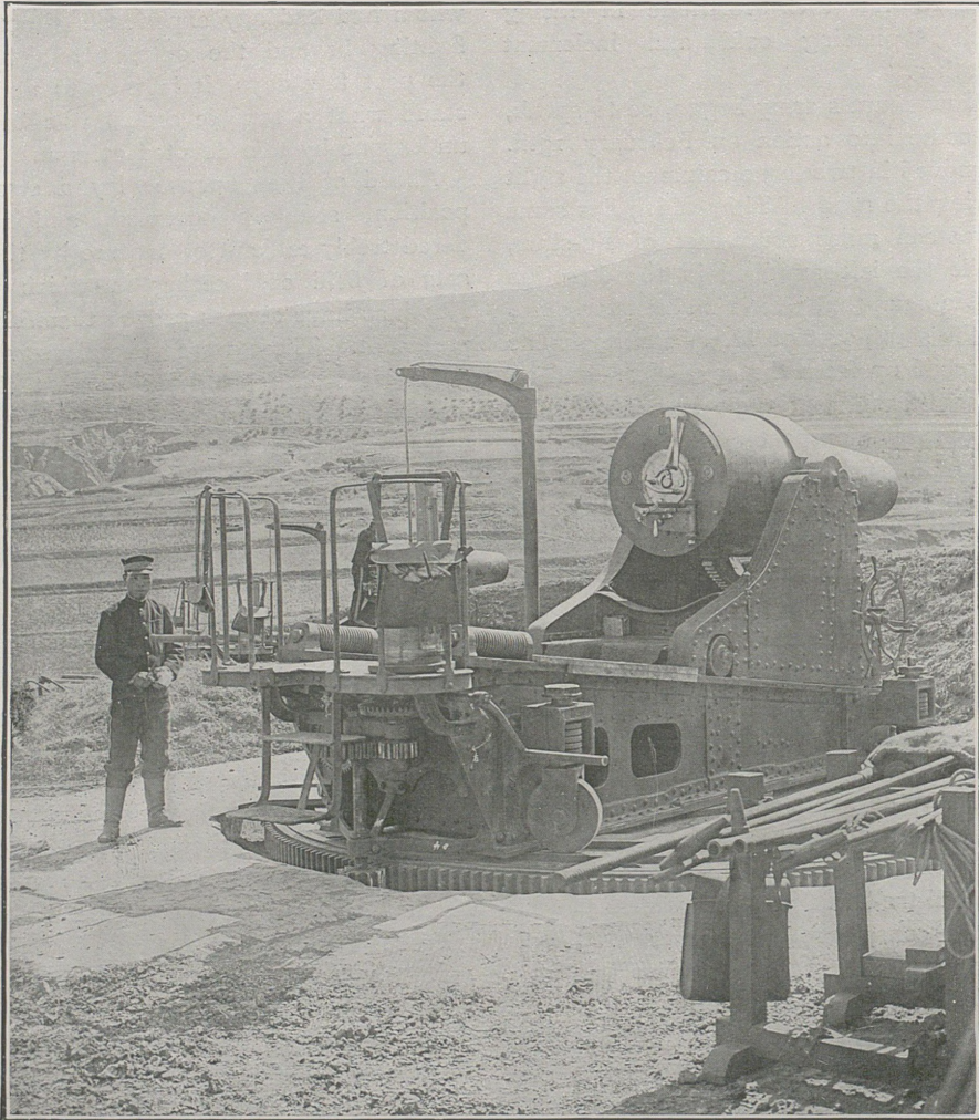
From Stereograph Copyright, 1905, by Underwood & Underwood, London and New York. ONE OF THE GREAT JAPANESE 11-INCH GUNS DRAGGED MANY MILES OVER ROUGH COUNTRY TO BE PLACED IN POSITION IN THE MANCHURIAN HILLS.
